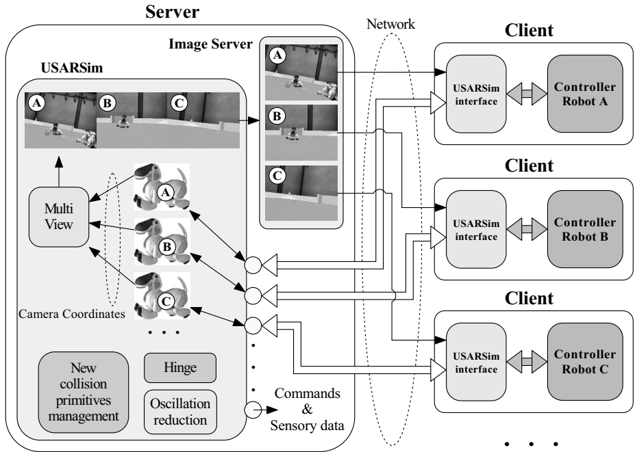
Fig. 1. Multi-Robot architecture
